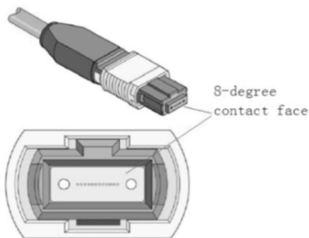
Figure 22 MTP/APC Cable
