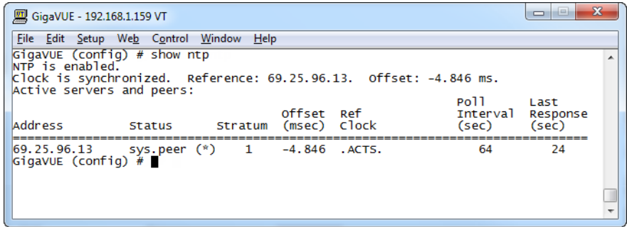
Figure 20 Checking NTP Status and Configuration
