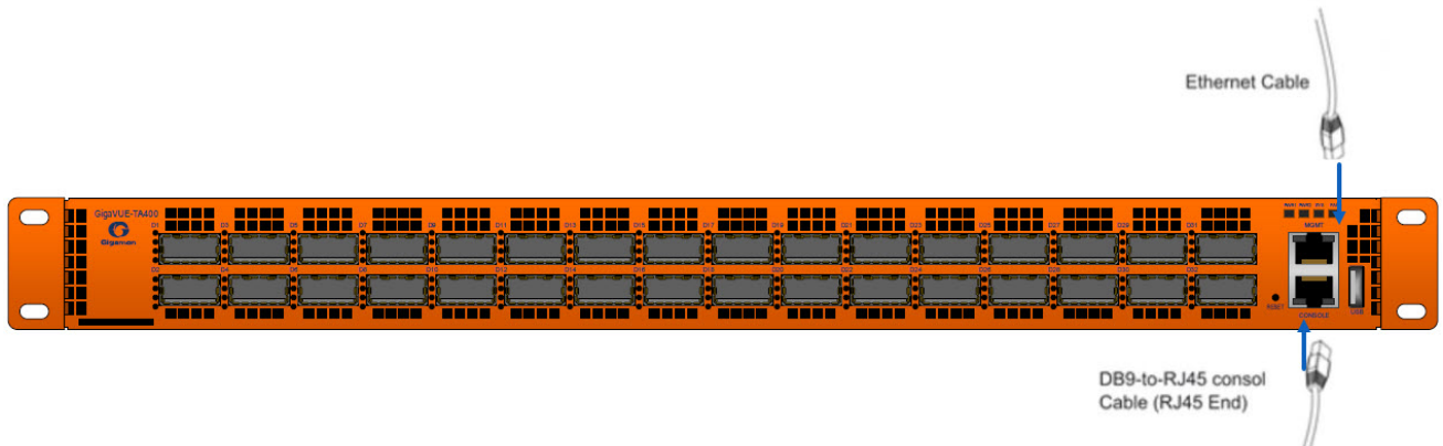
Figure 15 Connecting the Console and Management Ports
